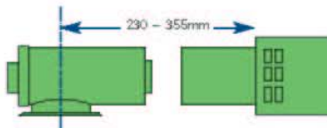
Flue Kit B, short horizontal flue
