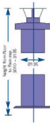
Flue Kit E, vertical flue
