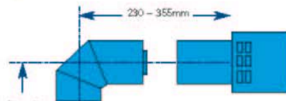
Flue Kit D, short horizontal high level flue
