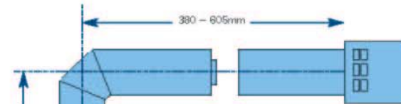
Flue Kit C, standard horizontal high level flue
