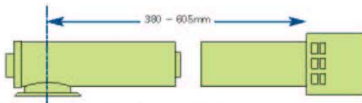
Flue Kit A, standard horizontal flue
